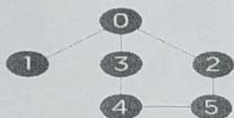
Graph with six nodes
